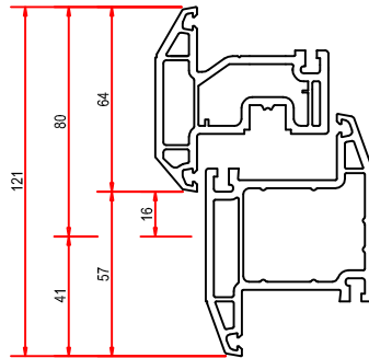
1468 / 1476 TYPICAL TRANSOM DETAIL WITH LARGER Z SECTION VENTED SECTION ON A FIXED UNIT
