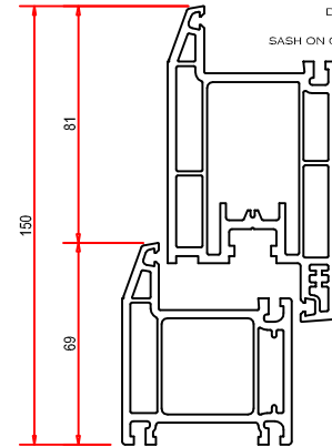
1478 / 1469 / 1478 TYPICAL MULLION DETAIL AT A VENTED BUTTMENT
