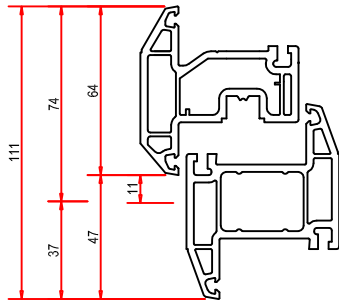
1478 / 1466 TYPICAL TRANSOM DETAIL WITH DEFAULT SASH VENTED SECTION ON A FIXED UNIT
