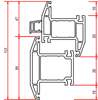
1461 / 1461 DEFAULT OUTER FRAME & SASH SASH ON OPEN IN DOORS
