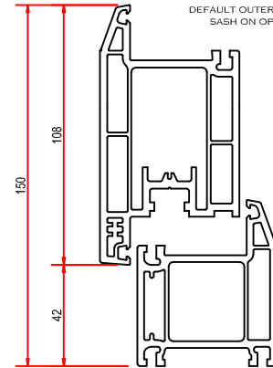
1460 / 0991 CILL TYPICAL CILL DETAIL & FIXED WINDOW
