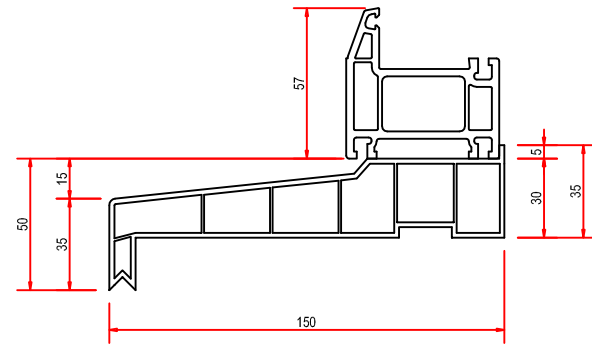
1460 / 0991 CILL TYPICAL CILL DETAIL & FIXED WINDOW
