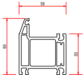
1478 / 1460 TYPICAL HEAD & JAMB DETAIL FOR VENTED OPTION
