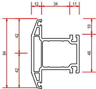
1470 OPTIONAL LARGER TRANSOM OR MULLION
