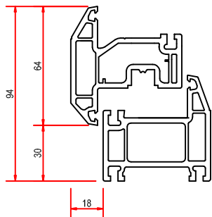
1478 / 1460 TYPICAL HEAD & JAMB DETAIL FOR VENTED OPTION
