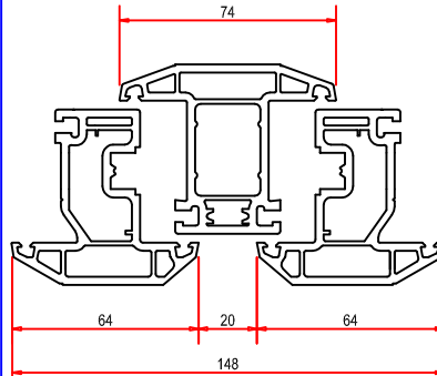
1468 / 1476 TYPICAL TRANSOM DETAIL WITH LARGER Z SECTION VENTED SECTION ON A FIXED UNIT
