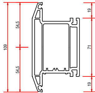
1471 OPTIONAL RAIL (MID-RAIL)
